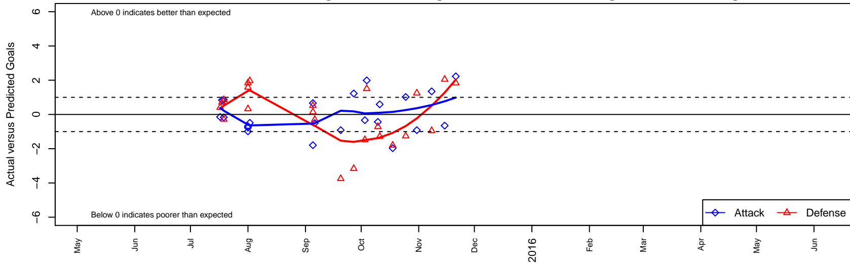
FME Xtreme B97 Dots are actual minus expected GF (blue circles) and GA (red triangles). Blue line is smoothed change in attack strength. Red is smoothed change in defense strength.
